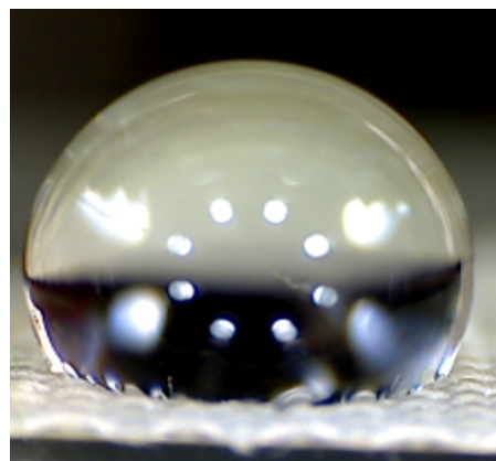
Fig. 6. Water droplet deposited on a cotton fabric treated with B/A-1/4 solution at 220 °C for 15 min.
