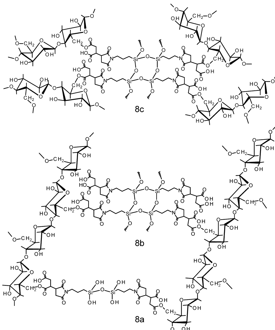
Fig. 8. Potential cross-linkage of the ladder-like polysilsesquioxane with the hydroxyl groups of the cellulose. (a) Single, (b) partial, (c) complete conversion of the vicinal carboxyl groups to ester linkages.
