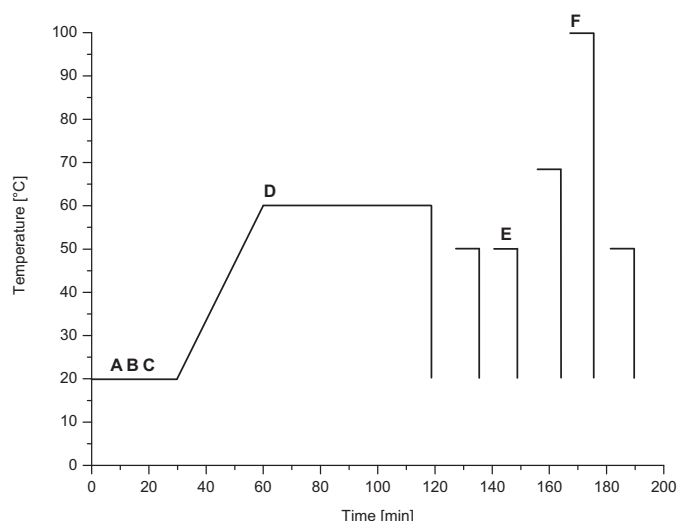
Fig. 2. Dyeing procedure. (A) Meropan NX, Biavin 109; (B) NaCl; (C) Na 2 CO 3 5.0 g/L, (D) NaOH 38° Bé, (E) acetic acid and (F) cotoblanco NSR.
