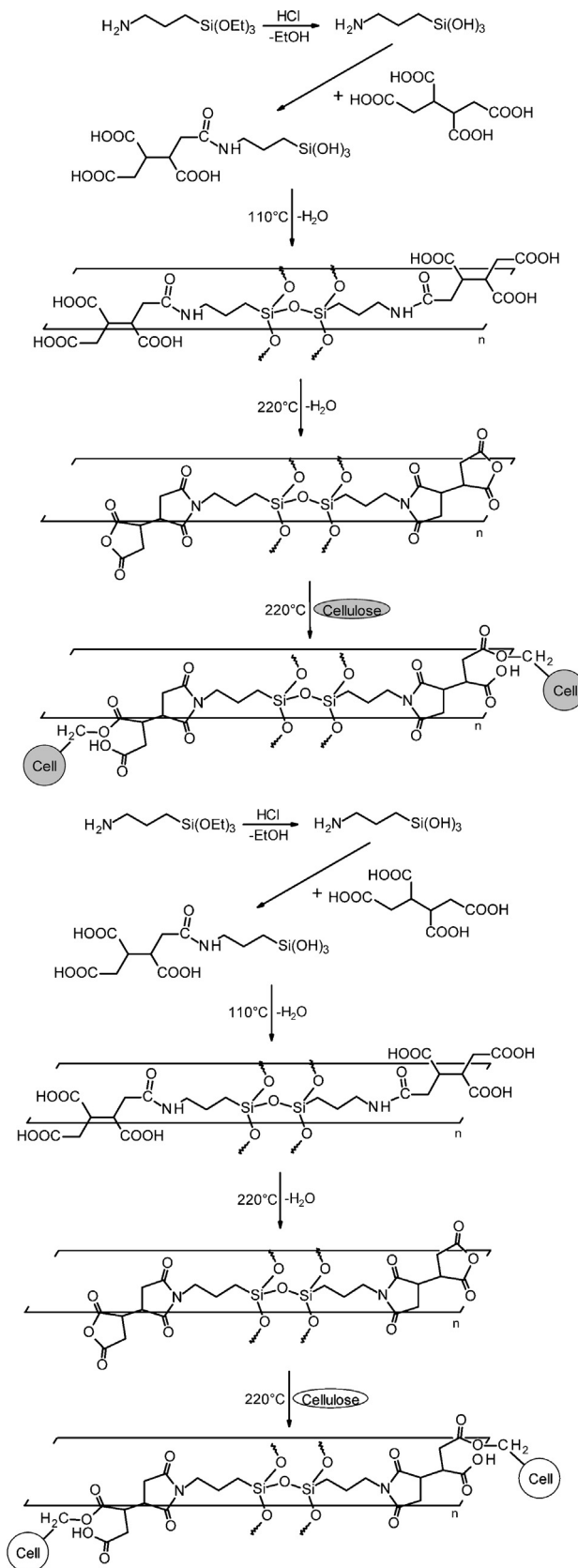
Fig. 7. Reaction scheme for the formation of the ladder-like polysilsesquioxane based on the reaction of APTES and BTCA at elevated temperature.
