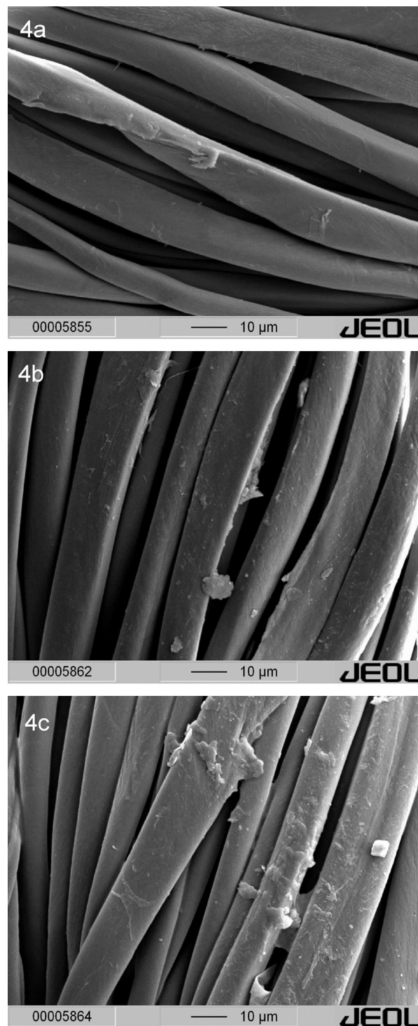
Fig. 4. SEM images of cotton raw material (a), and BTCA/APTES treated cotton samples: B/A-1/1-220-15 (b) and BA-1/4-220-15 (c).
