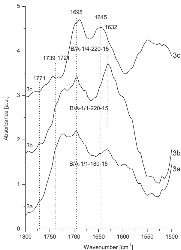
Fig. 3. FT-IR spectra of B/A-1/1-180-15 (a), B/A-1/1-220-15 (b) and B/A-1/4-220-15 (c).
